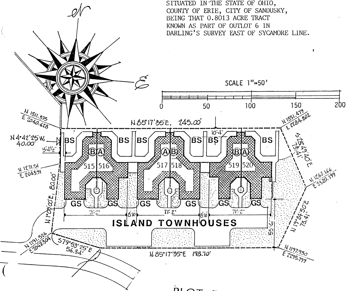
PLOT PLAN SCALE 1"=50'
